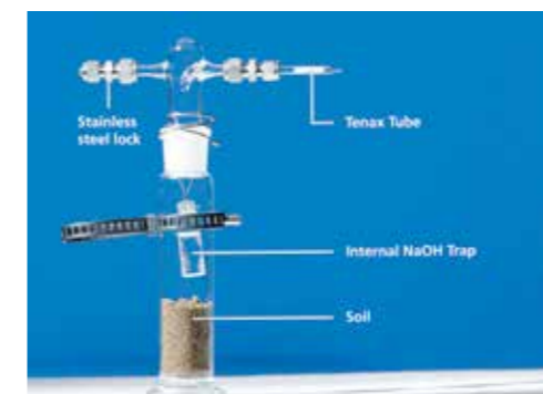
Improved closed setup for testing volatile chemicals in soil (Shrestha et al. 2018).
